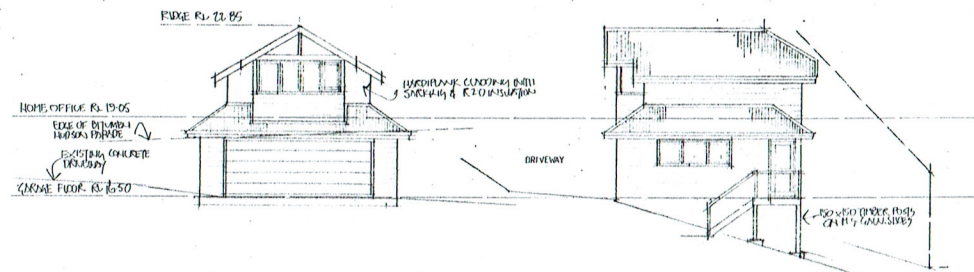
NORTH-EAST ELEVATION
