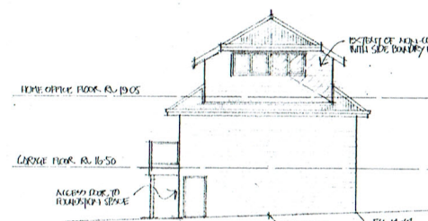
SOUTH-WEST ELEVATION
