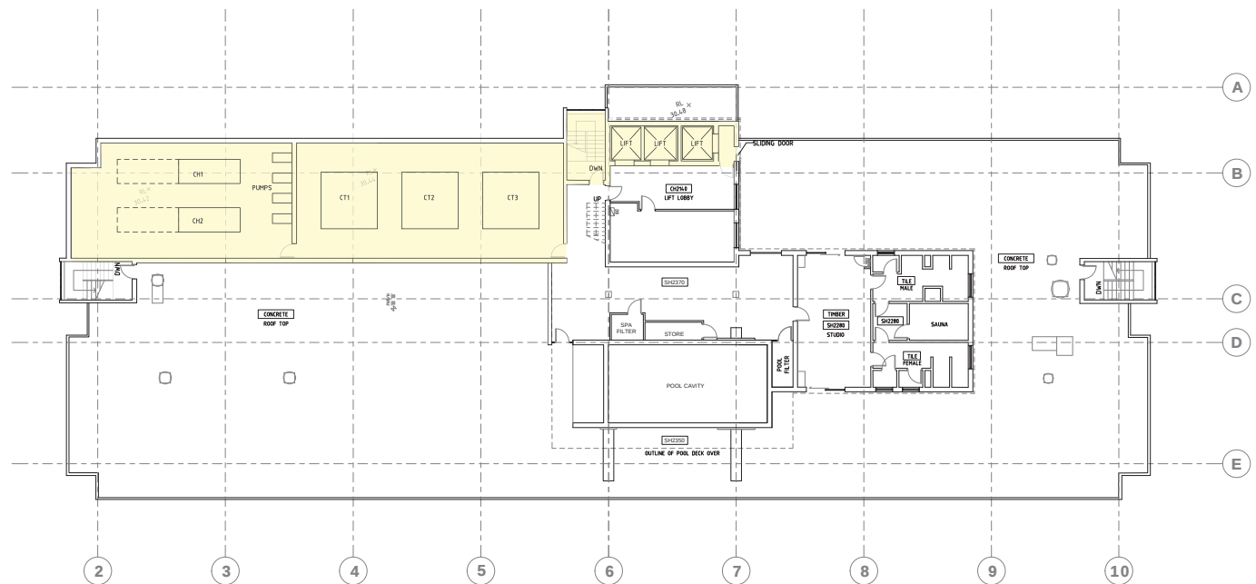
LEVEL 8 PLANT AND LIFT LAYOUT
