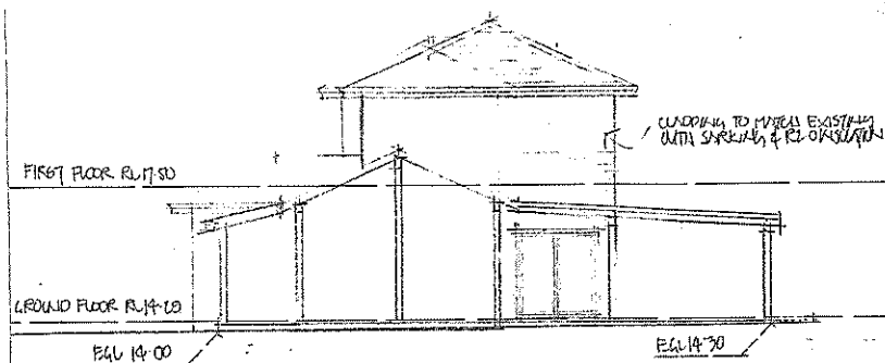
NORTH ELEVATION
