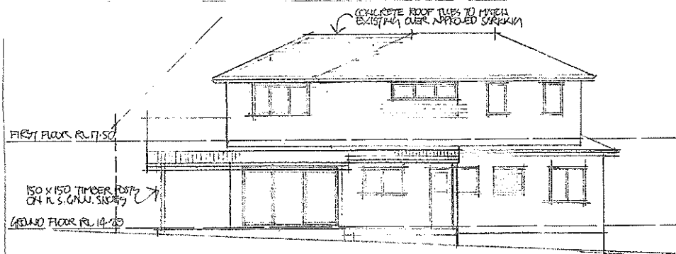
WEST ELEVATION
