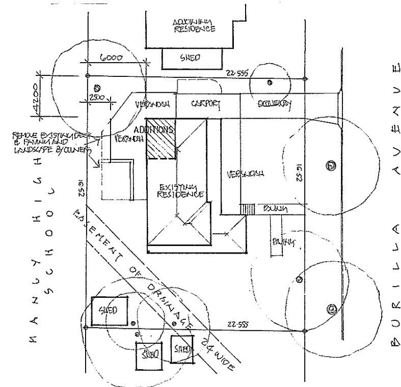
SITE PLAN
