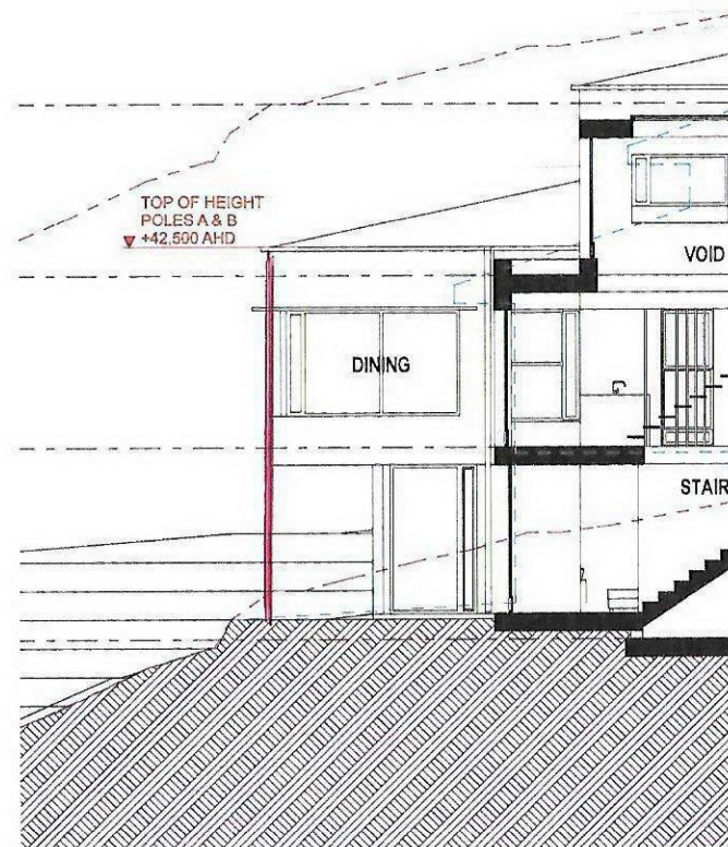
② Section A
