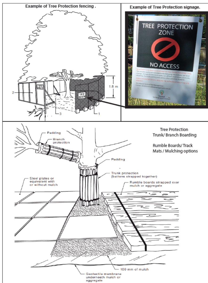
Figure 3 - Example of Tree Protection
