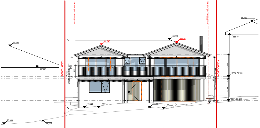
E.1 HILMA ST ELEVATION (EAST)
