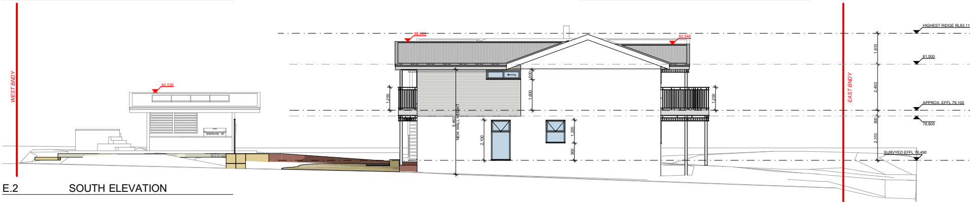
E.2 SOUTH ELEVATION
