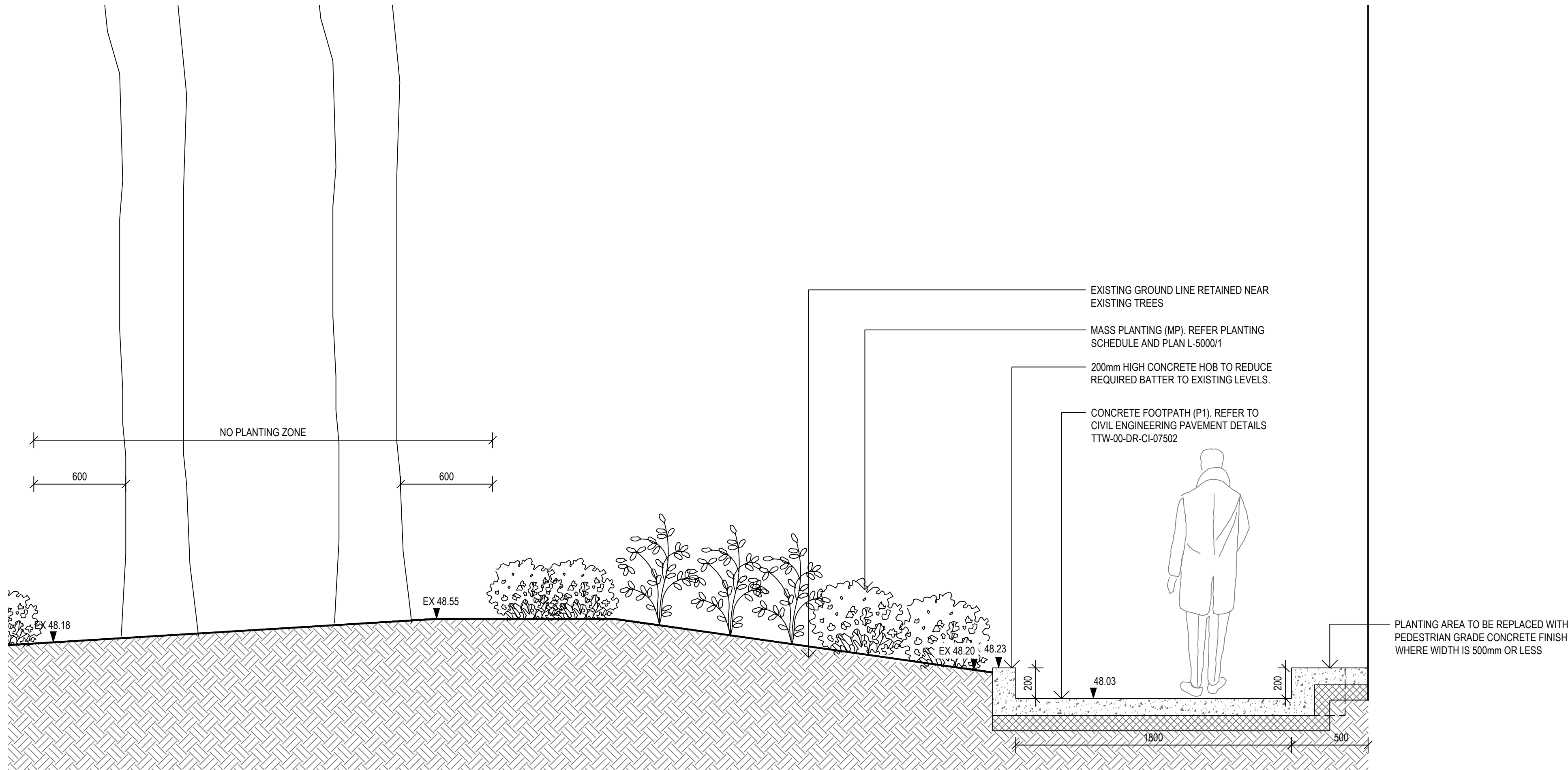
01 6001 1:20 TYPICAL CONCRETE HOB TO FOOTPATH
