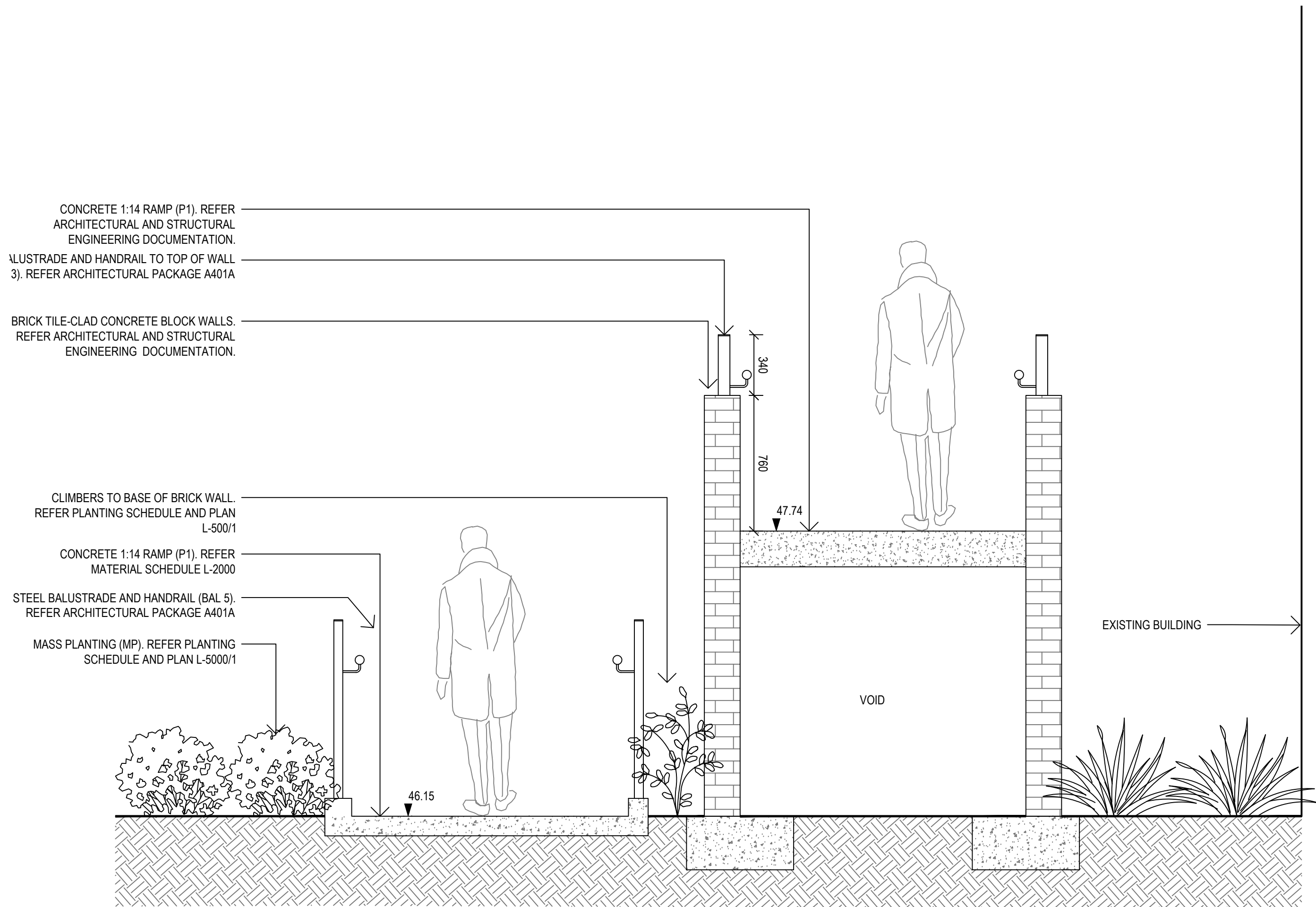
02 6001 1:20 RAMP TO THEATRE ENTRY
