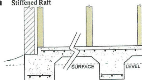
Fig. 1 Stiffened Raft
