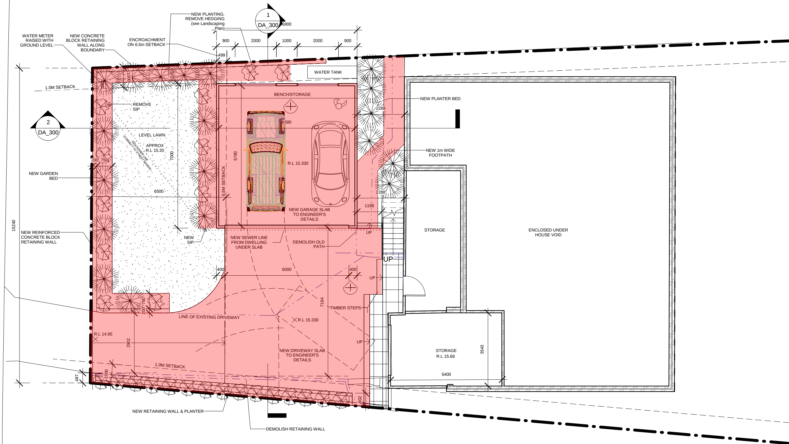
1 GROUND 1 : 100
