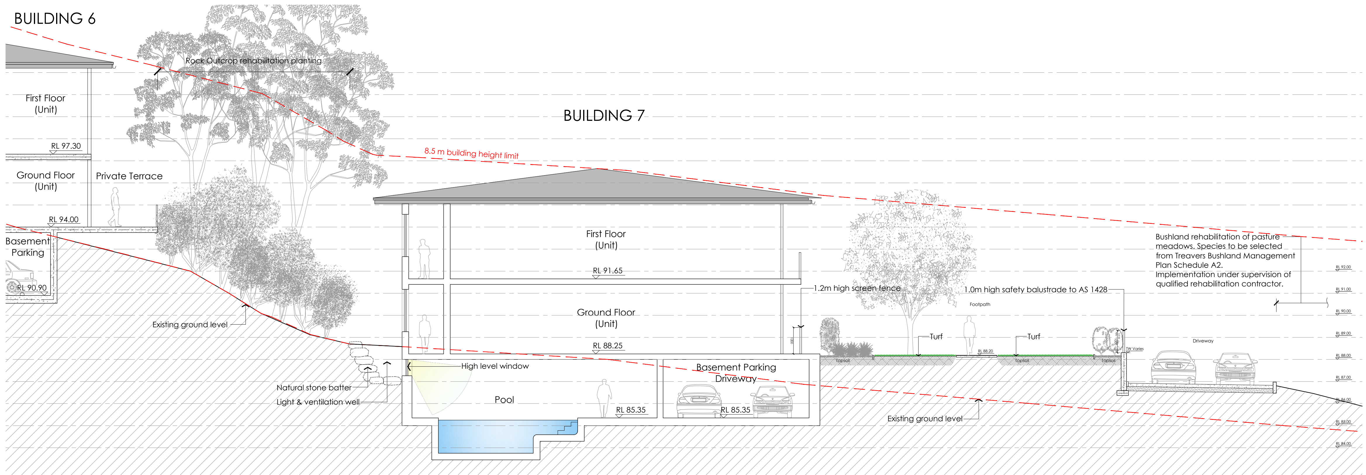
Section A-A Scale 1: 100 @ B1
