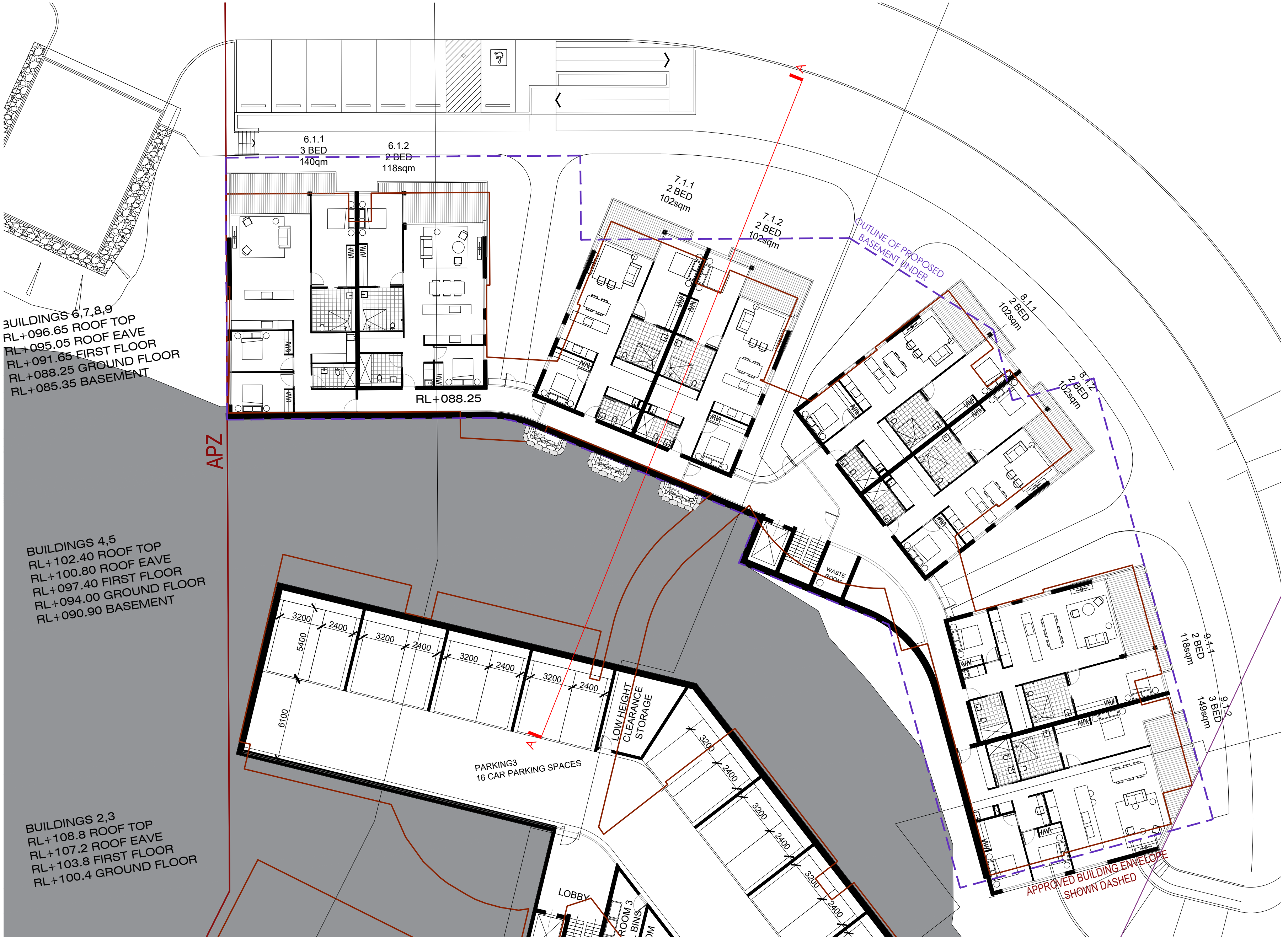
Layout Plan - RL 88.25 Ground Floor Scale 1: 200 @ B1
