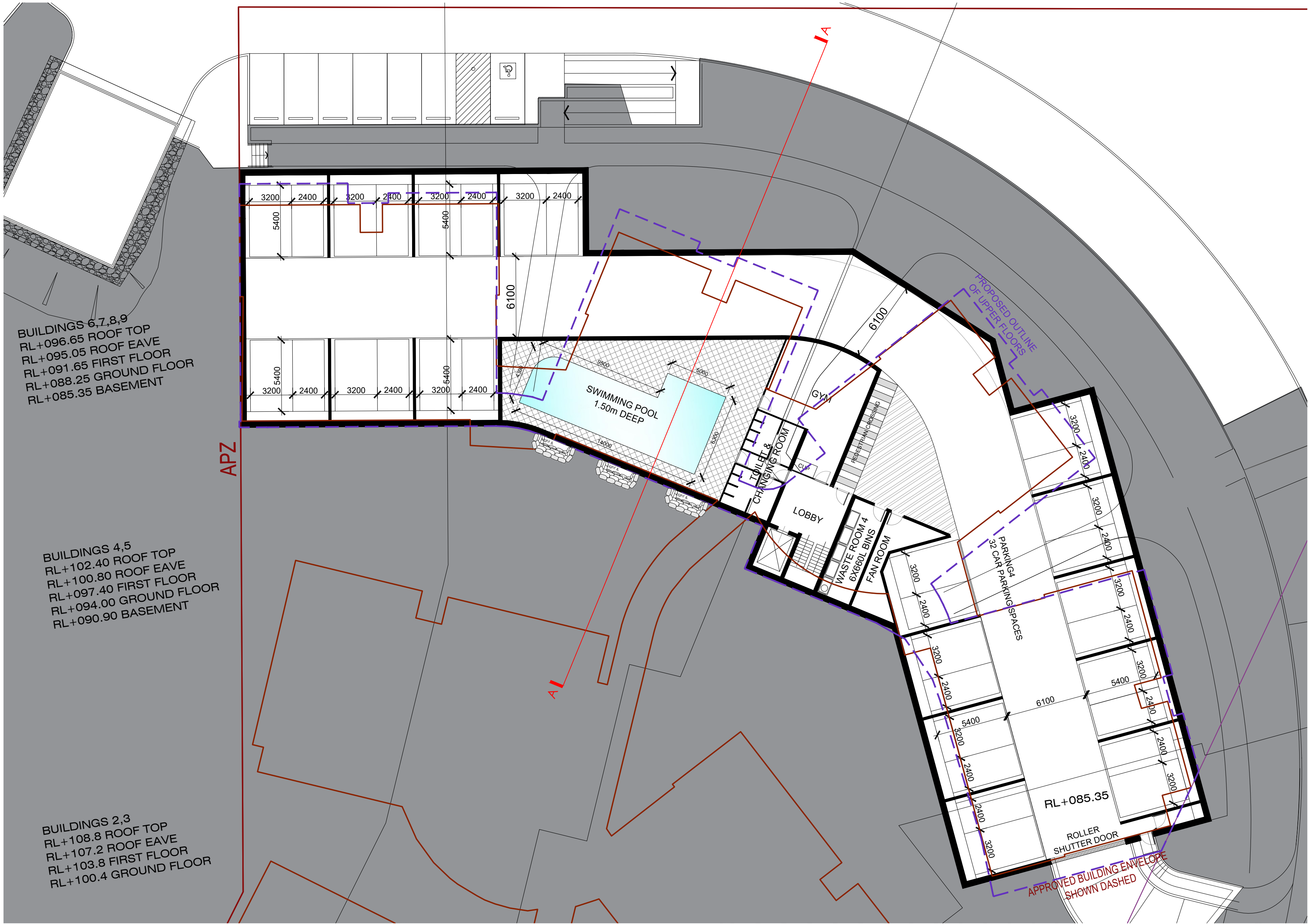
Layout Plan - RL 85.35 Basement Scale 1: 200 @ B1
