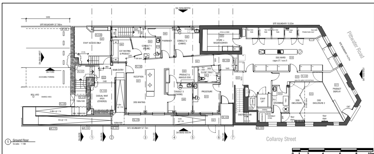
Figure 2. Proposed Architectural Plan
