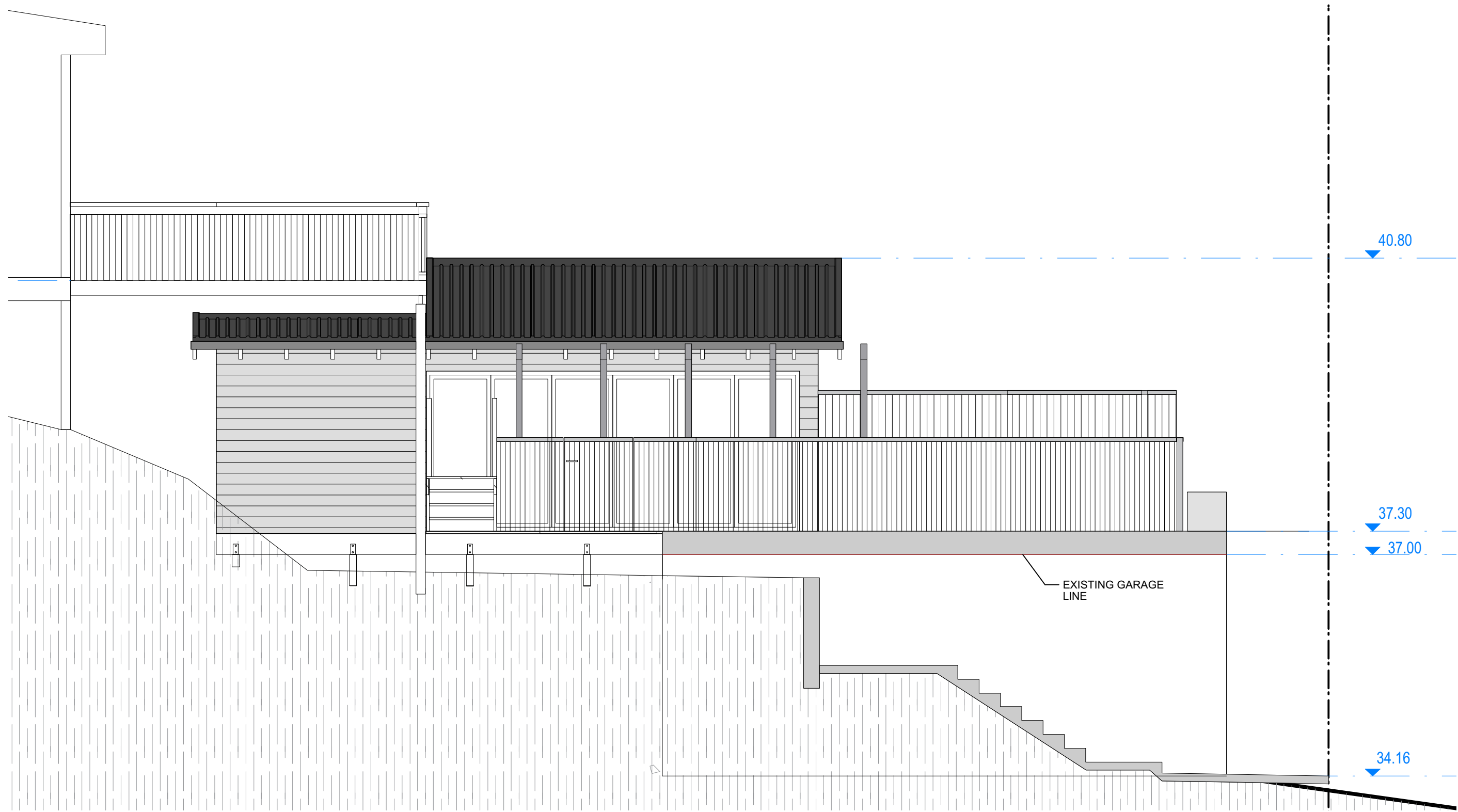
Elevation South 1:50@A1 1:100@A3.
