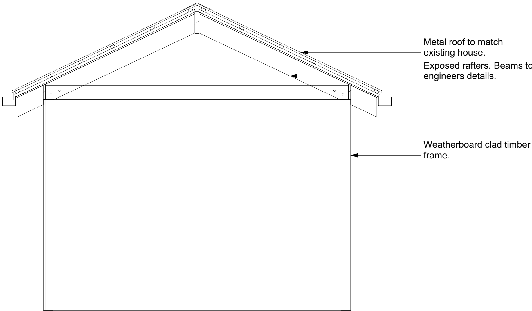
Cabana Section 1:25@A1 1:50@A3.
