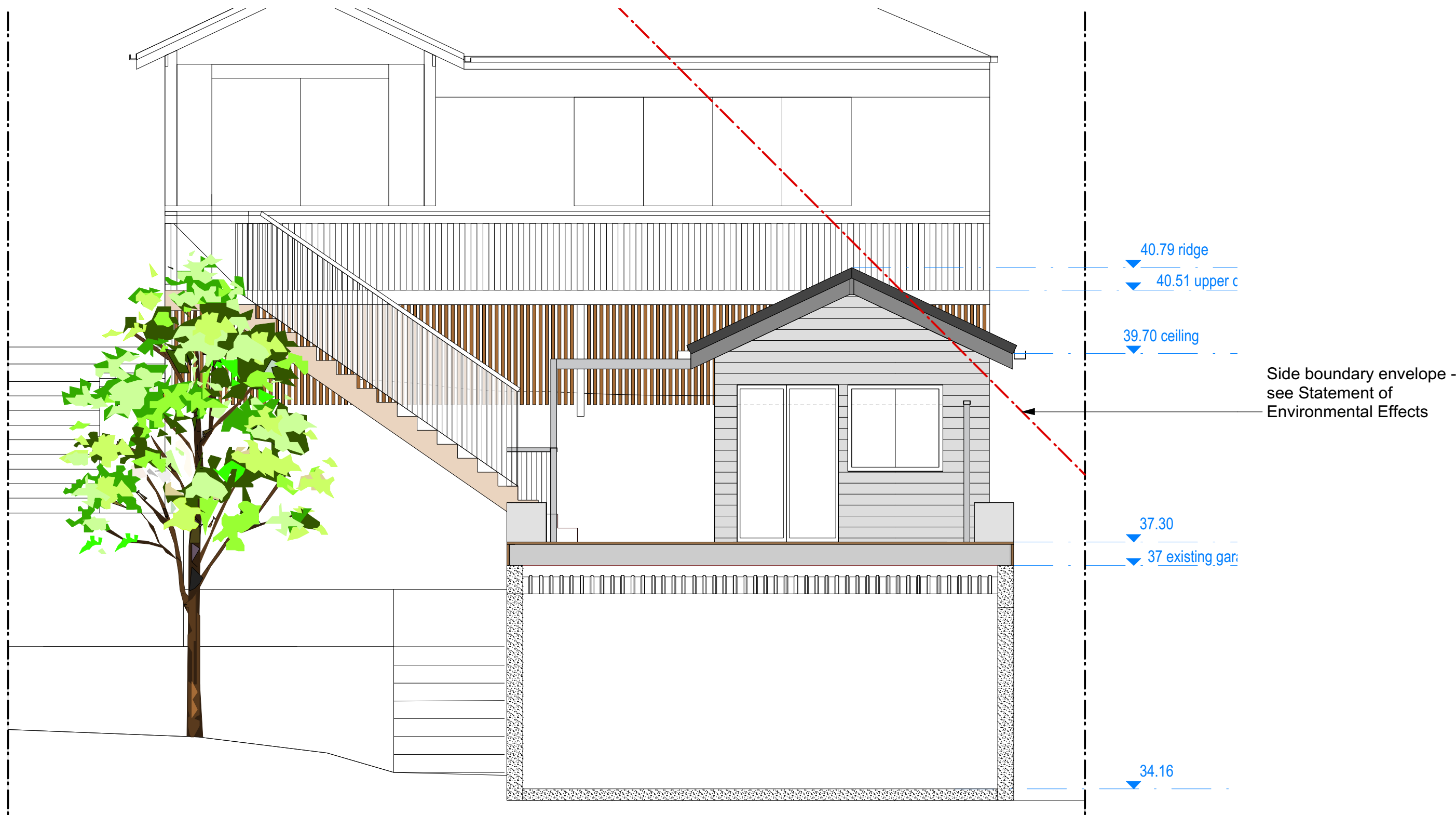
Cross Section 1:50@A1 1:100@A3.
